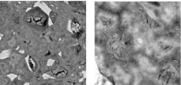
Ettringite cores forming into aged cement pastes. Right picture is a 2 years old paste subjected to sulfate attack. One clearly sees the ettringite cores forming within the C-S-H.
