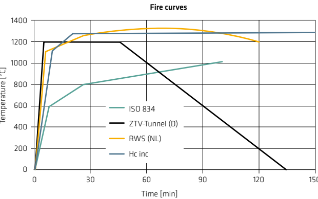
These fire exposure rating curves all simulate the temperature profile of a tunnel fire. The example of the RWS curve defines the maximum exposure which can be expected in the worst case scenario: Defined as a fire of a tank truck with a load capacity of 50m³ which is 90% full of liquid hydrocarbon fuel (petrol).
