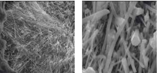
Classic form of sulfate attack associated with ettringite or gypsum formation. Flurly of ettringite rods grown in mature cement pastes subjected to external sulfate solutions.
