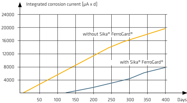
The Sika Research Department in Zurich tested the anticorrosive effect of Sika® FerroGard® on cracked concrete beams. The specimens were produced in accordance with ASTM G 109 and were cyclically treated with road salts. Periodic measurement of the corrosion current confirms the protective effect of Sika® FerroGard®.
