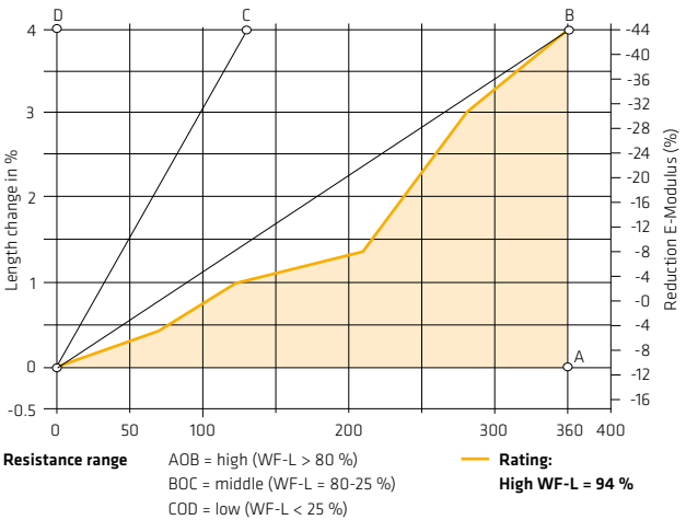
Artificially introduced air voids, caused by an air entrainer, generate space for expansion in the concrete structure to allow for the roughly 10% increase in volume when water freezes to become ice. In test BE II according to D-R 400, the test prisms are subject to alternating loads between +20°C and -20°C, the change in length is measured and judged between three ranges of durability (low / middle / high). Calculation according to ASTM C666.
