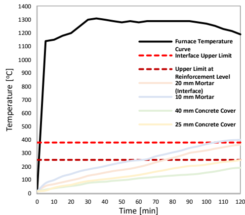
Figure 2. Results of testing under the RWS curve with 10 mm and 20 mm of fire protection mortar (NTUA).
