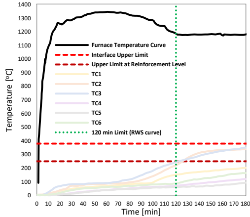
Figure 4. Results of testing under the RWS curve with 13 mm and 26 mm of the fire protection mortar (Hagerbach).
