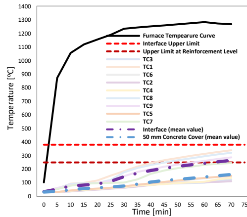
Figure 5. Results of testing under the RWS curve for a 15 mm layer of the fire protection mortar in the Panagopoula railway tunnel.
