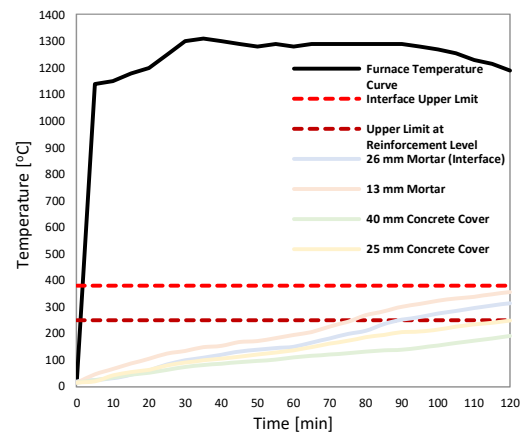
Figure 3. Results of testing under the RWS curve for 13 mm and 26 mm of the fire protection mortar (NTUA).
